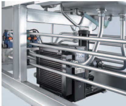
Additional air cooler for the hydraulic buffer fluid
