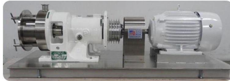
STANDARD CHARLOTTE "SD" MODEL SANITARY GREASE PRODUCTION MILL
