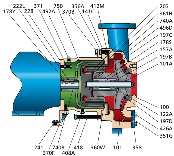
3298 L Close-Coupled
