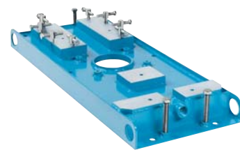
ENHANCED FEATURE FABRICATED STEEL Upgraded ANSI baseplate designed to maximize pump operation life and ease installation by meeting API-minded chemical pump users toughest requirements.
